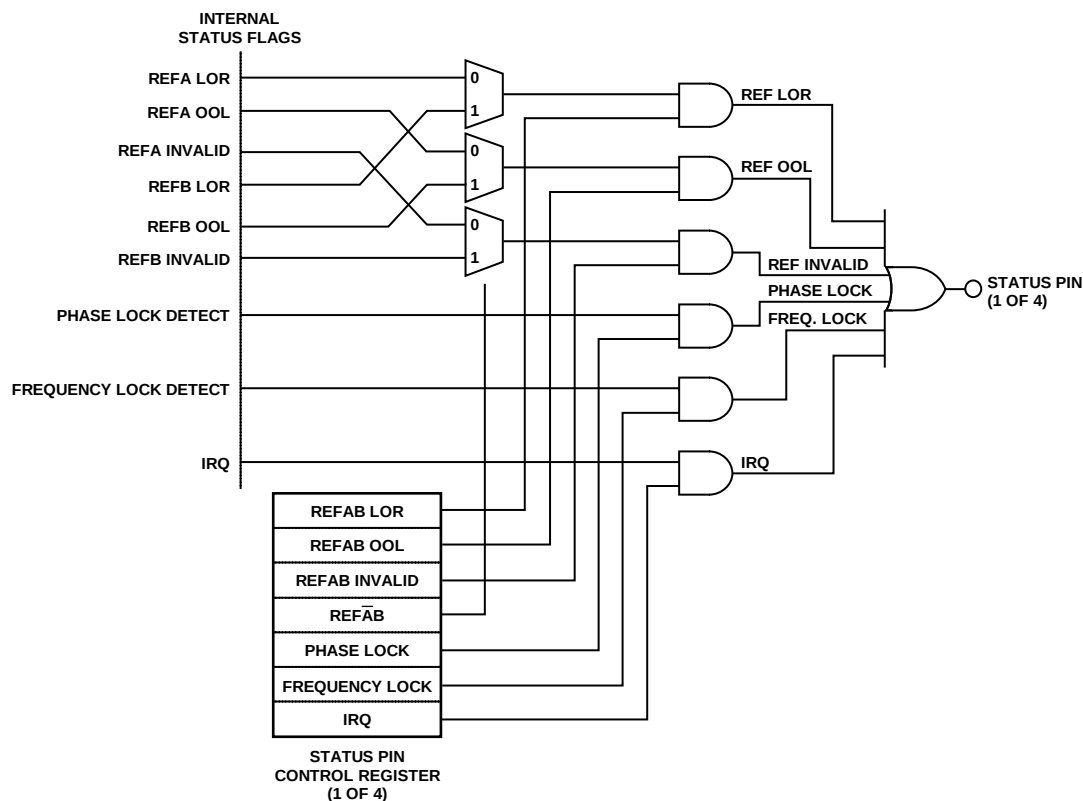
Figure 49. Status Pin Control
