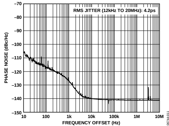
Figure 11. Additive Phase Noise at HSTL Output Driver, \text{SYSCLK} = 500 \text{ MHz} ( \text{SYSCLK PLL Disabled} ), f_{\text{REF}} = 10.24 \text{ MHz} , f_{\text{OUT}} = 20.48 \text{ MHz} , \text{DPLL Loop BW} = 1 \text{ kHz}
