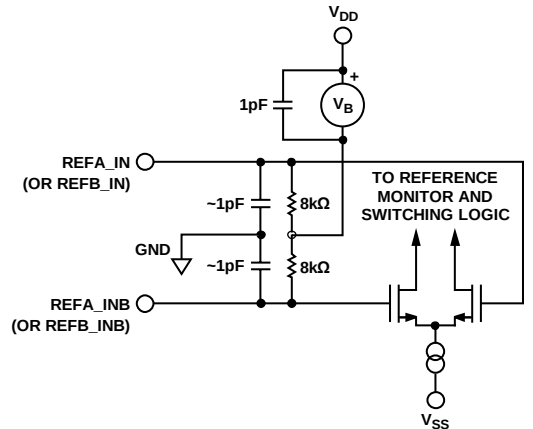
Figure 41. Reference Inputs
