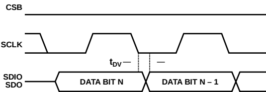
Figure 56. Timing Diagram for Serial Control Port Register Read
