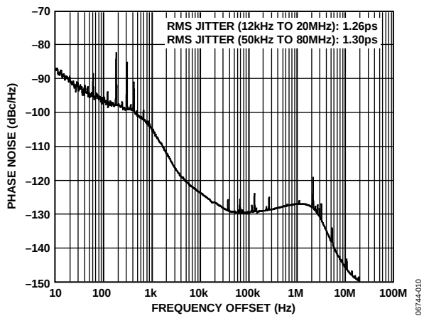
Figure 10. Additive Phase Noise at HSTL Output Driver, \text{SYSCLK} = 1 \text{ GHz} ( \text{SYSCLK PLL Enabled and Driven by a 25 MHz Fox Crystal Oscillator} ), f_{\text{REF}} = 19.44 \text{ MHz} , f_{\text{OUT}} = 155.52 \text{ MHz} , \text{DPLL Loop BW} = 1 \text{ kHz}
