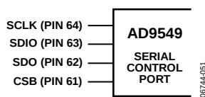
Figure 51. Serial Control Port
