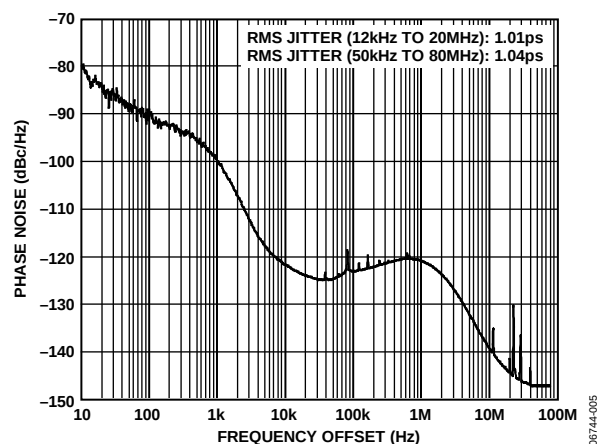
Figure 5. Additive Phase Noise at HSTL Output Driver, SYSCLK = 1 GHz (SYSCLK PLL Enabled and Driven by R&S SMA100 Signal Generator at 50 MHz), f_{REF} = 19.44 MHz, f_{OUT} = 311.04 MHz, DPLL Loop BW = 1 kHz
