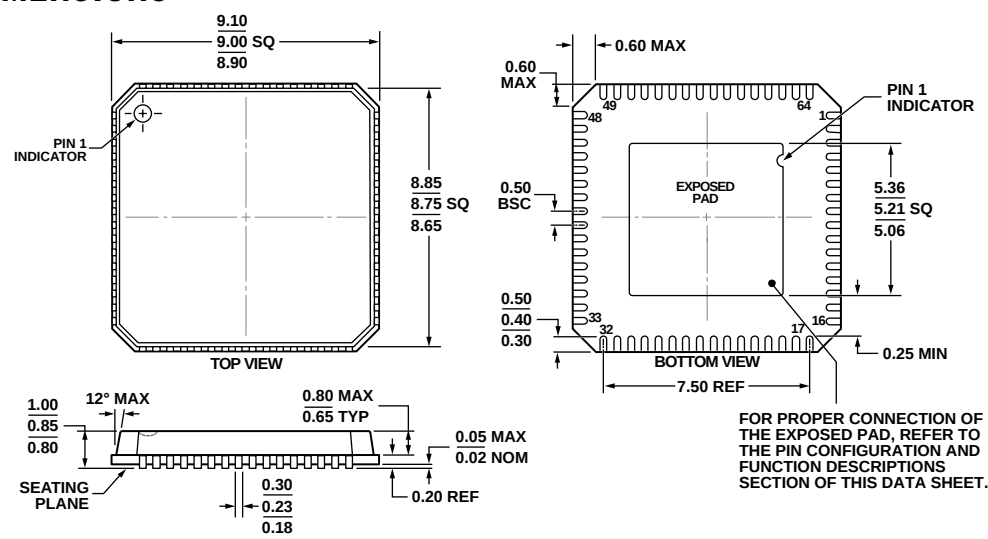
COMPLIANT TO JEDEC STANDARDS MO-220-VMMD-4 Figure 60. 64-Lead Lead Frame Chip Scale Package [LFCSP_VQ] 9 mm × 9 mm Body, Very Thin Quad (CP-64-7) Dimensions shown in millimeters
