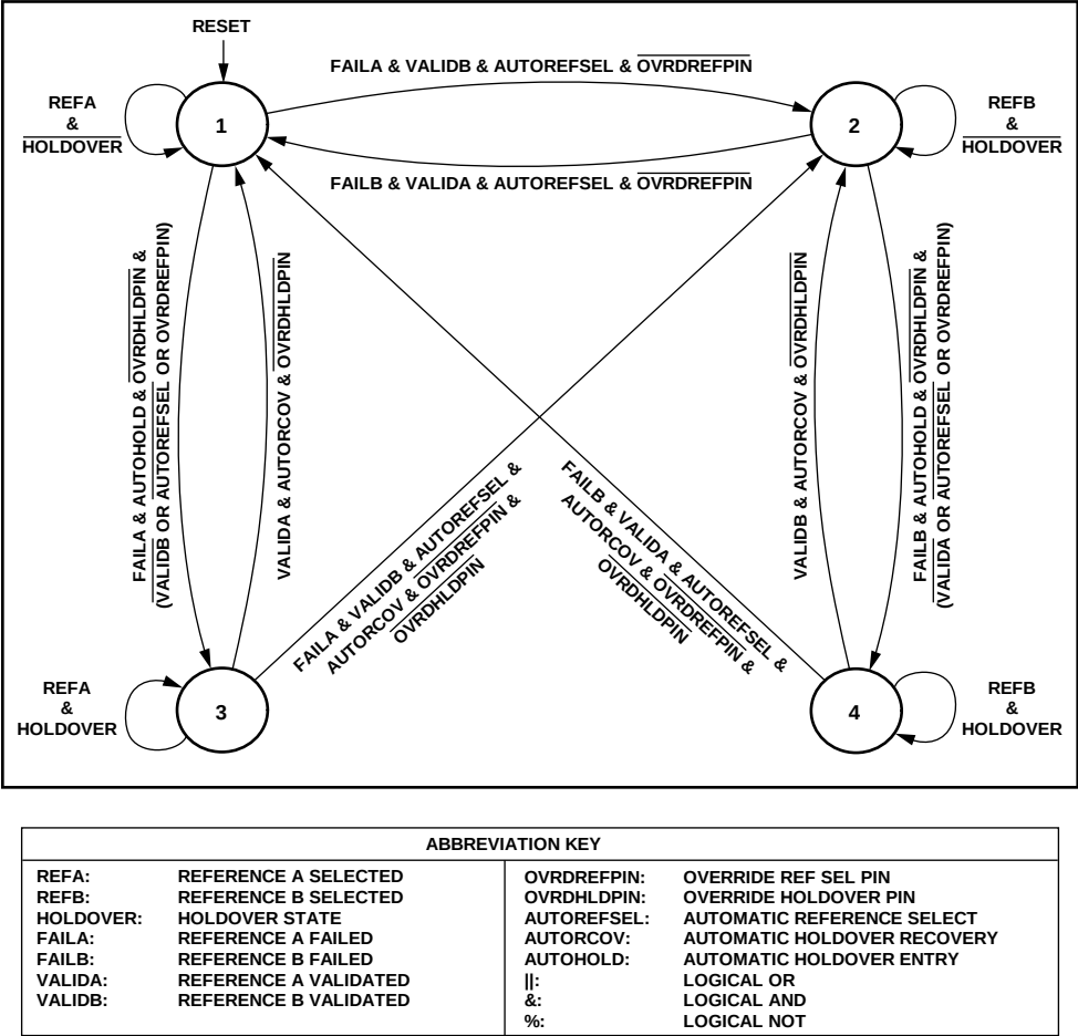
Figure 37. Holdover State Diagram
