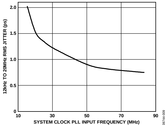
Figure 9. 12 kHz to 20 MHz RMS Jitter vs. System Clock PLL Input Frequency, \text{SYSCLK} = 1 \text{ GHz} , f_{\text{REF}} = 19.44 \text{ MHz} , f_{\text{OUT}} = 155.52 \text{ MHz}
