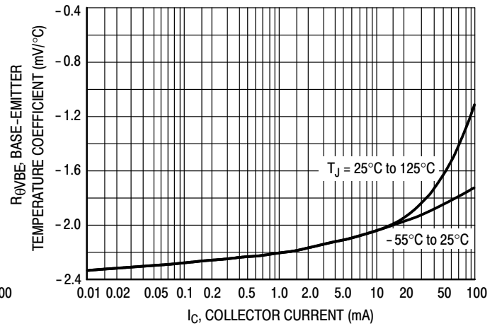
Figure 10. Temperature Coefficients
