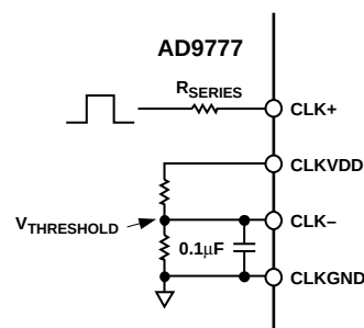
Figure 43. Single-Ended Clock Driving Clock Inputs
