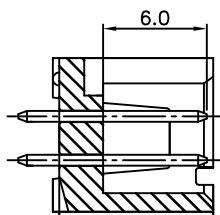
SECTION A-A WITHOUT CAP
