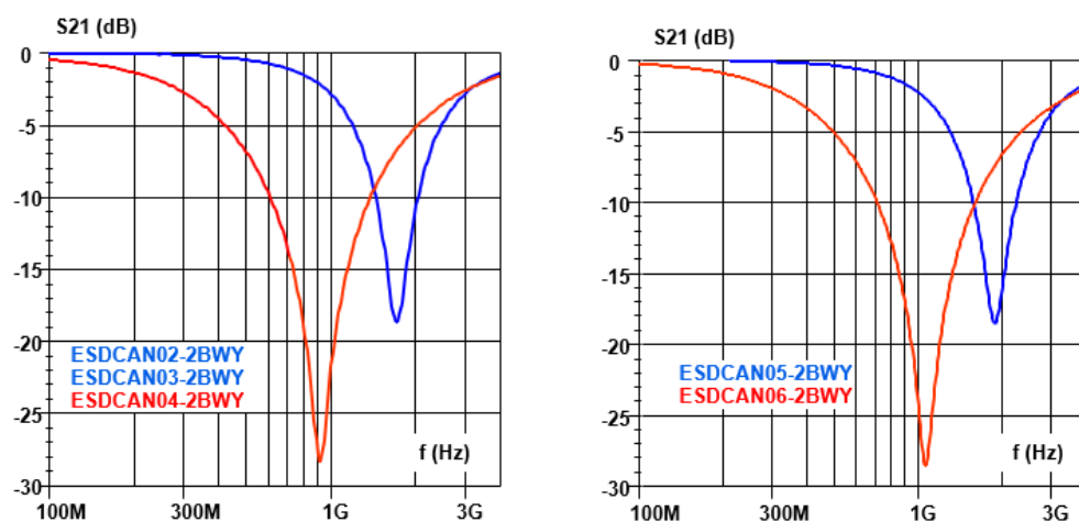
Figure 13. S21 attenuation
