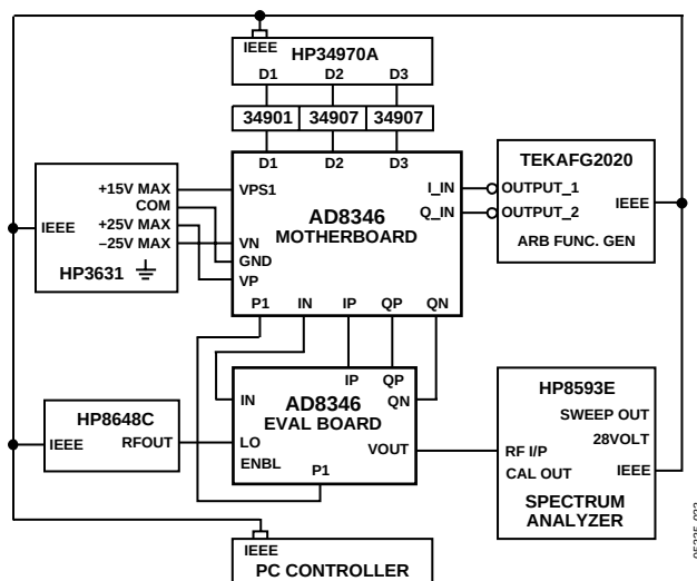
Figure 33. Evaluation Board SSB Test Setup
