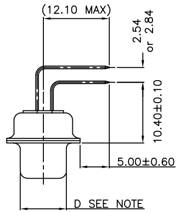
LAYOUT OF 50 POS.CONNECTOR
