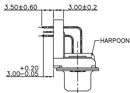
HARPOON WITH PLASTIC BRACKET
