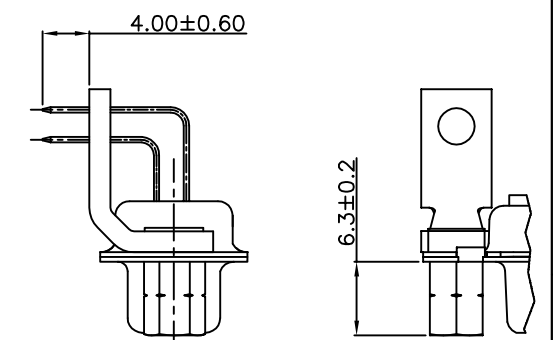
VIEW WITH RIVETED FEMALE SCREW &amp; METAL BRACKET
