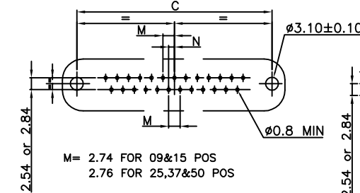
PCB DRILLING DETAIL - 09 TO 37 POS
