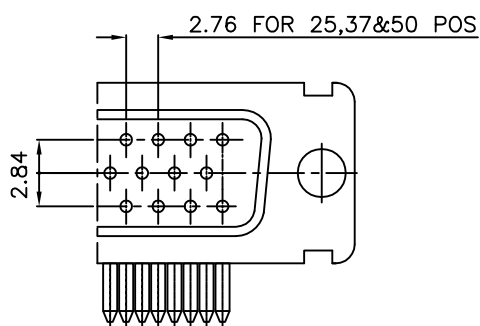
LAYOUT OF 50 POS.CONNECTOR
