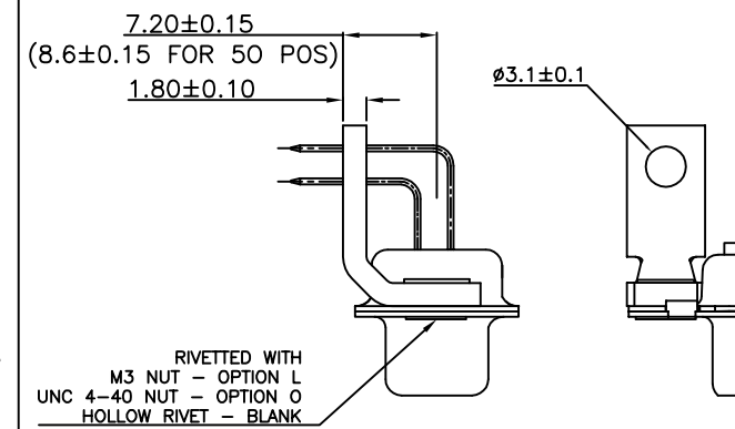
VIEW WITH RIVET &amp; METAL BRACKET
