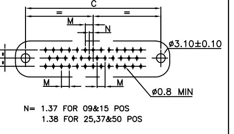
PCB DRILLING DETAIL - 50 POS
