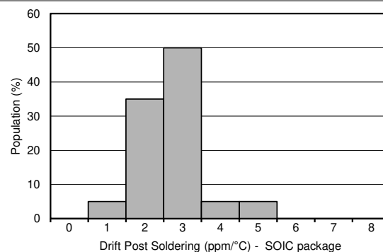
Figure 7-6. Drift Post Soldering Distribution, SOIC Package
