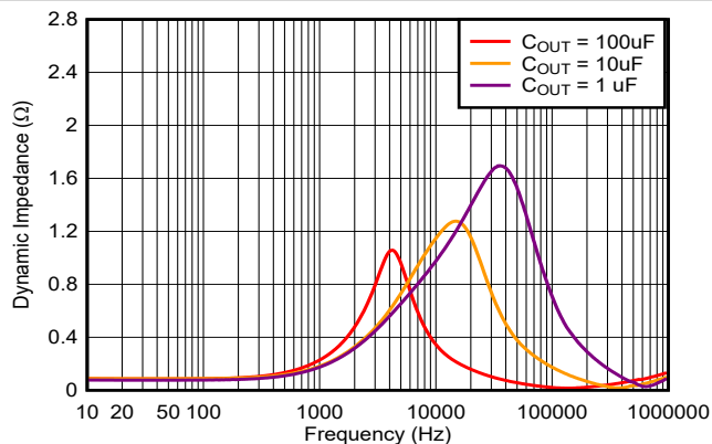
Figure 6-40. Output Impedance
