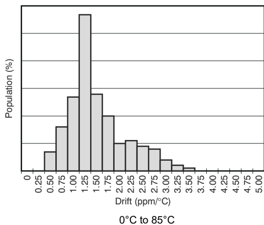
Figure 6-1. Temperature Drift
