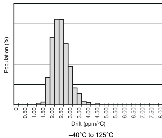
Figure 6-2. Temperature Drift
