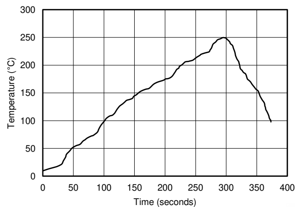
Figure 7-1. Reflow Profile
