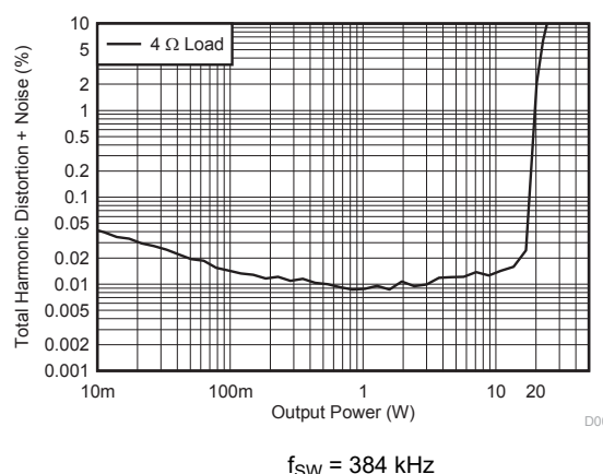
Figure 7-6. THD+N vs Power
