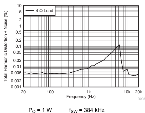
Figure 7-4. THD+N vs Frequency
