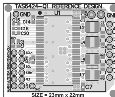
PCB AREA
