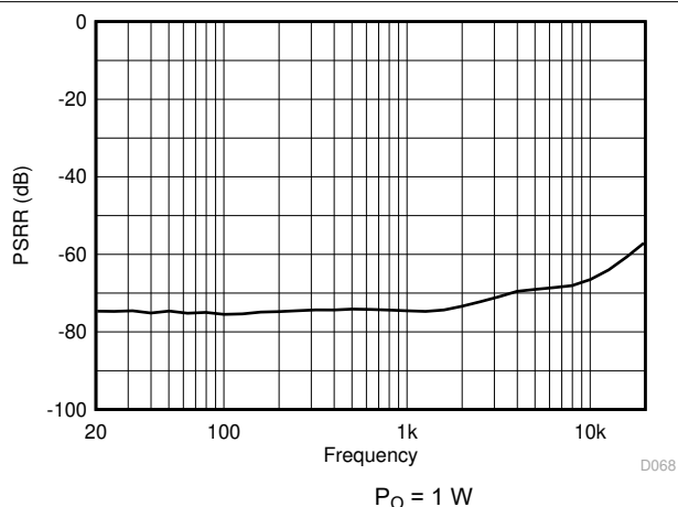
Figure 7-2. PVDD PSRR vs Frequency
