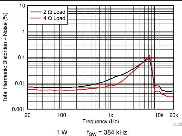
Figure 7-18. PBTL THD+N vs Frequency
