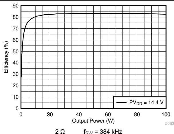
Figure 7-13. PVDD Power Efficiency vs Total Output Power
