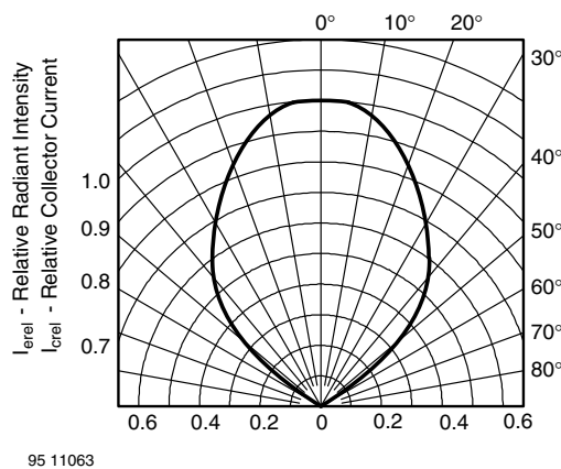
Fig. 10 - Relative Radiant Intensity/Collector Current vs. Angular Displacement
