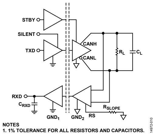
Figure 30. Switching Characteristics Measurements
