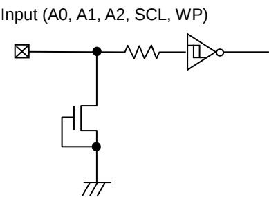
Figure 50. Input Pin Circuit Diagram
