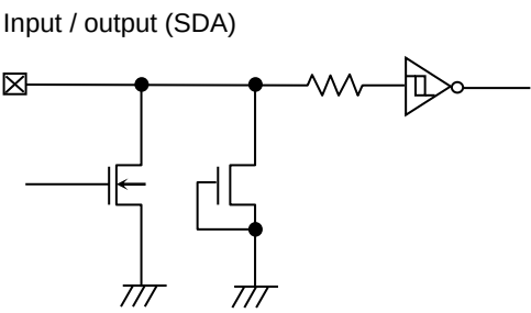
Figure 51. Input / Output Pin Circuit Diagram
