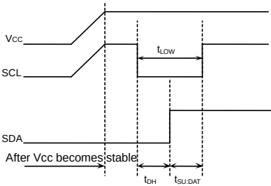
Figure 53. When SCL= 'H' and SDA= 'L'
