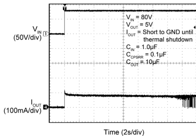
Thermal-Shutdown Response
