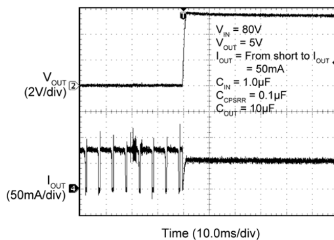
V_{OUT} Recovery from Thermal Shutdown
