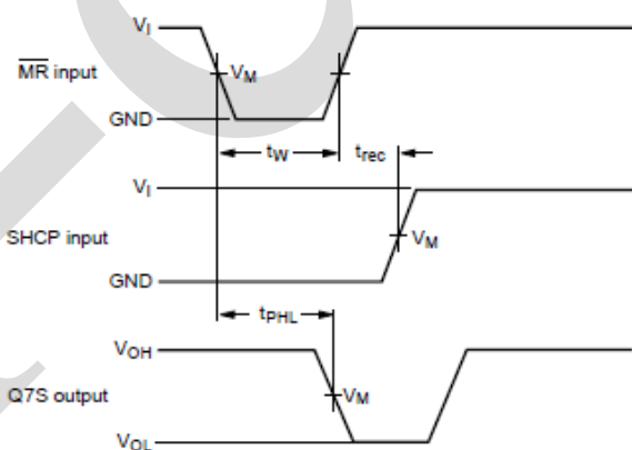
Figure 9. Master reset to output propagation delays
