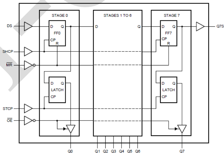
Figure 3. Logic diagram
