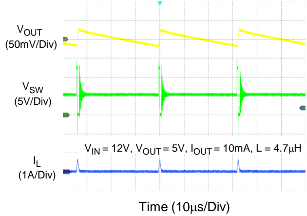
Output Ripple as IOU = 10mA
