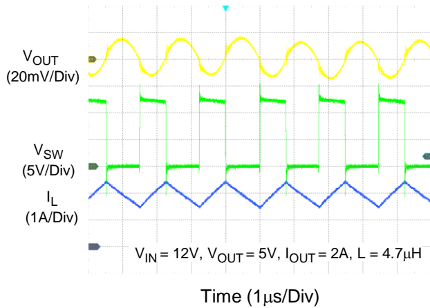
Output Ripple as IOU = 2A
