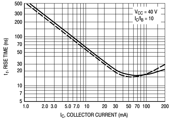
Figure 7. Rise Time
