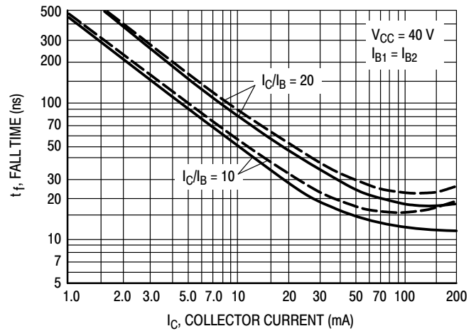
Figure 9. Fall Time
