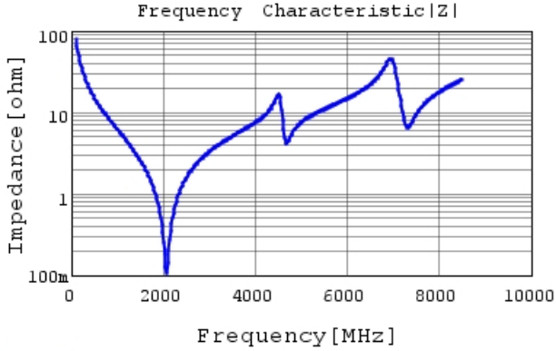
GCQ1555C1H200JB01 |Z| DC0V, 25degC
