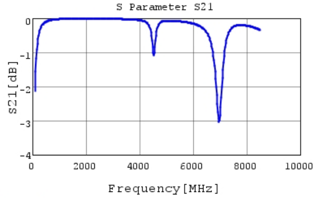
GCQ1555C1H200JB01 S21 DCOV, 25degC
