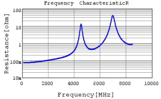
GCQ1555C1H200JB01 R DC0V, 25degC
