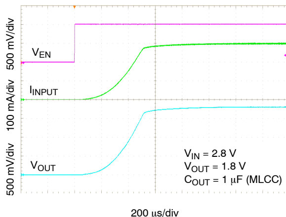
Figure 29. Enable Turn-on Response – I_{OUT} = 300 mA, Slow Option – C
