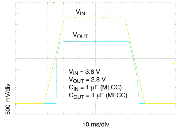
Figure 43. Turn-on/off - Slow Rising V_{IN} - I_{OUT} = 300\text{ mA}
